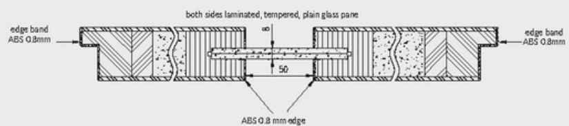
Horizontal cross-section of rebated VETRO E doors
